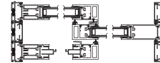
Frame Detail
